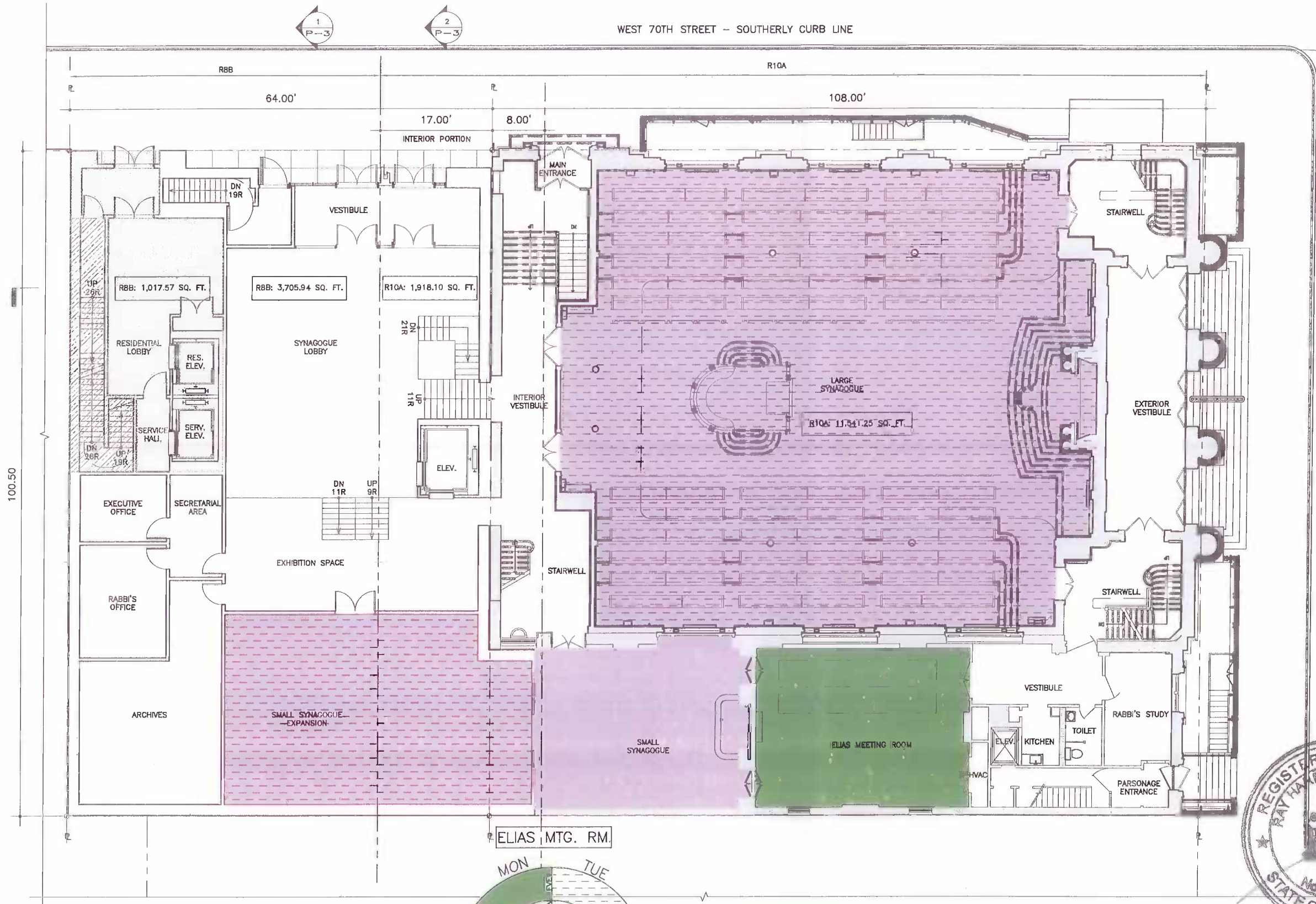
1 PLAN FIRST FLOOR SCALE: 1/16" = 1'-0"
