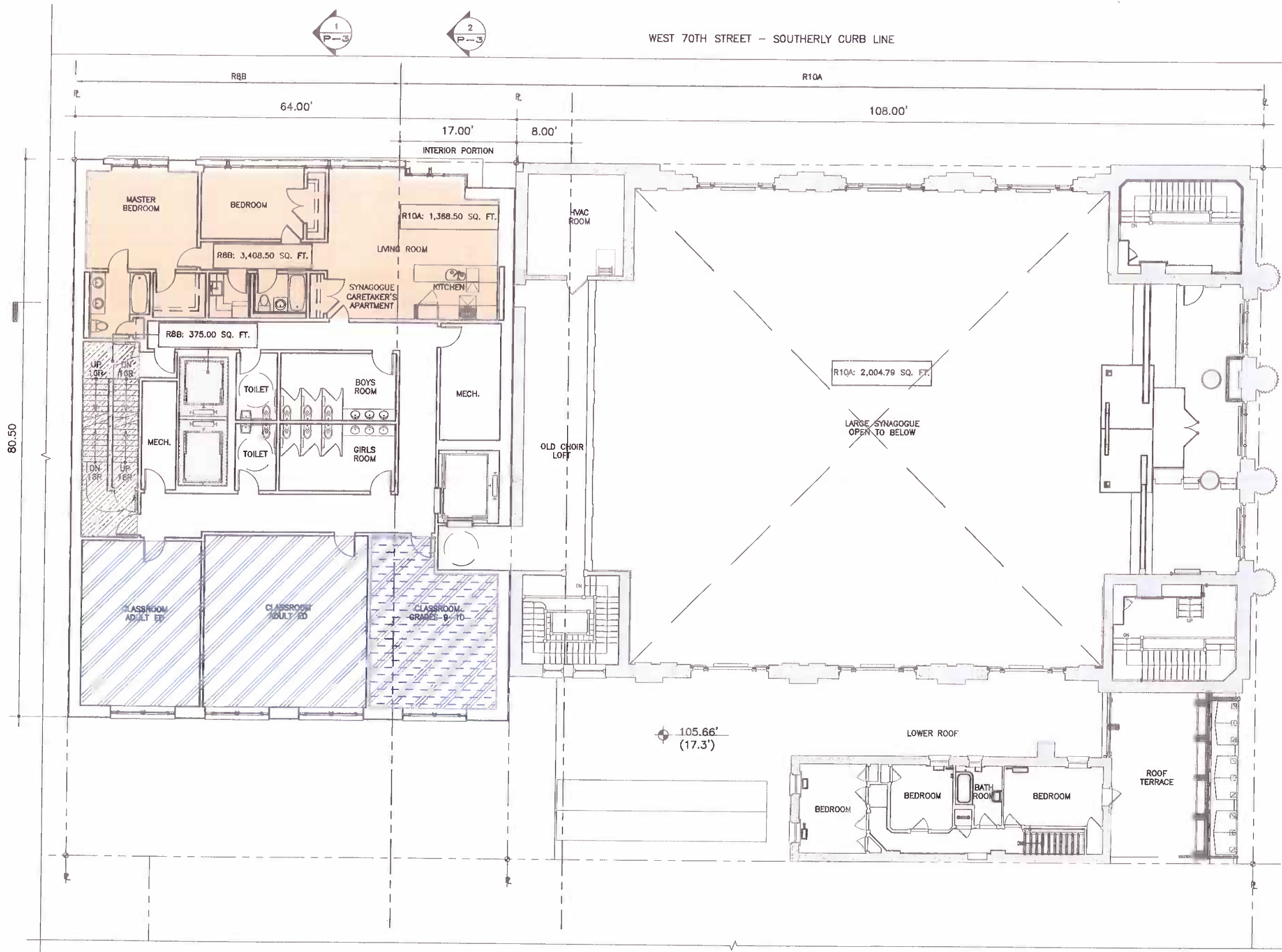
1 PLAN FOURTH FLOOR SCALE: 1/16" = 1'-0"
