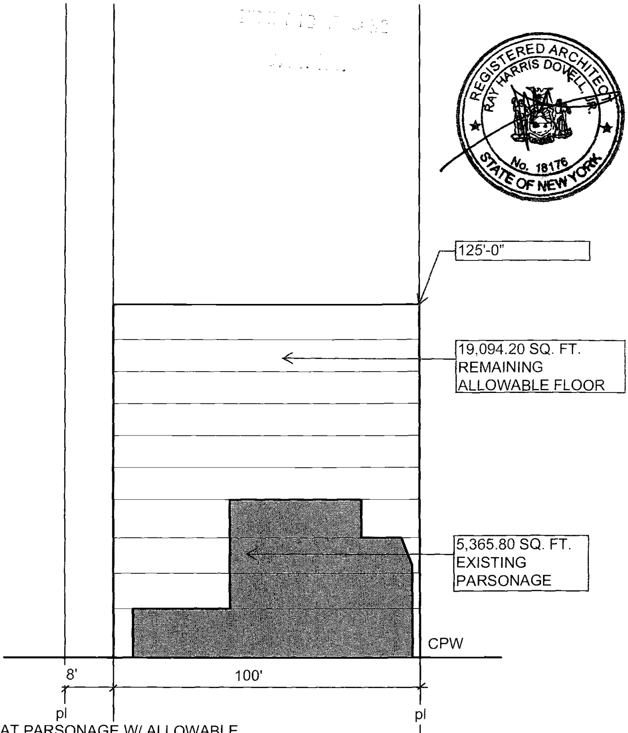
SECTION AT PARSONAGE W/ ALLOWABLE FLOOR AREA FOR PARSONAGE PARCEL
